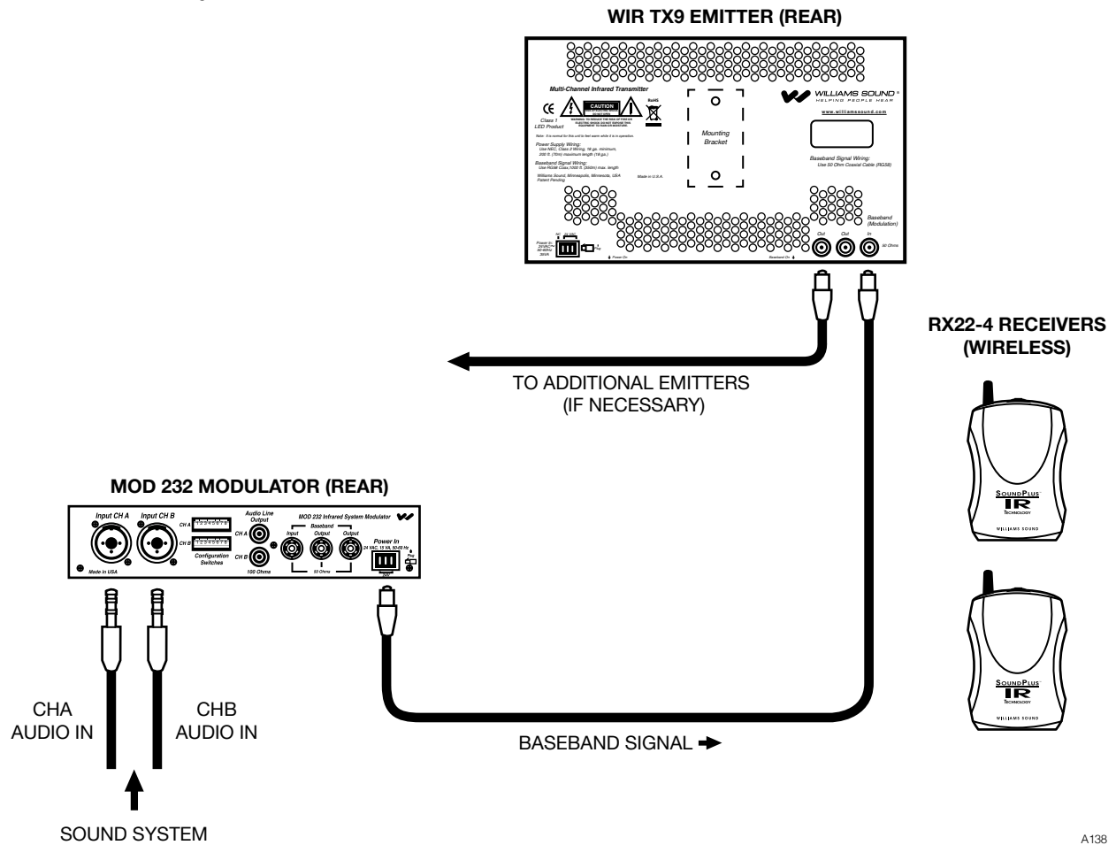
Fig. 12: Two-Channel System
